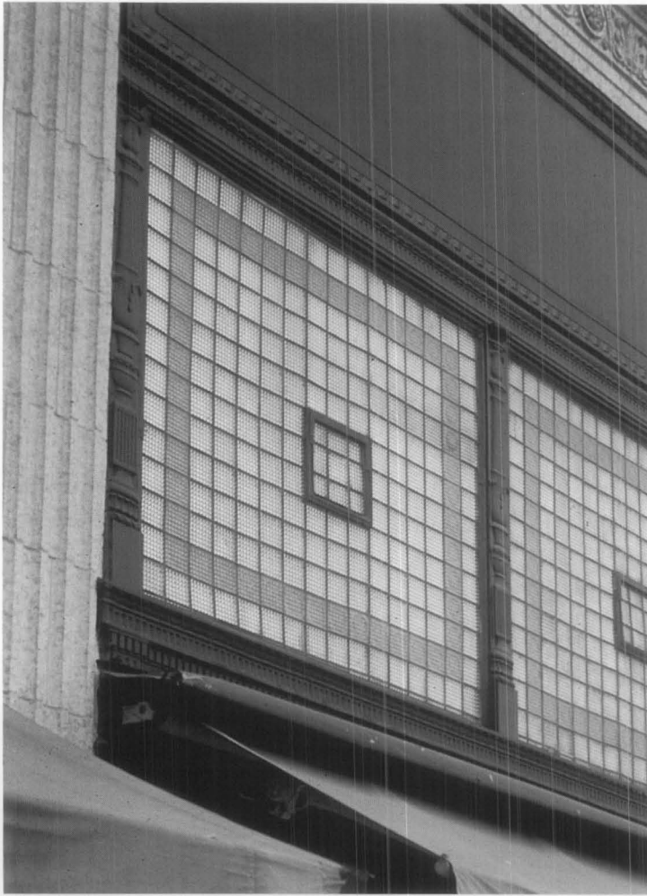
Figure 7. Rebuilt transoms featured prismatic glass tiles and vents that were original to the building. The decorative border of “trademark” tiles was incorporated into the reglazed assembly. Photo: Chad Randl.
