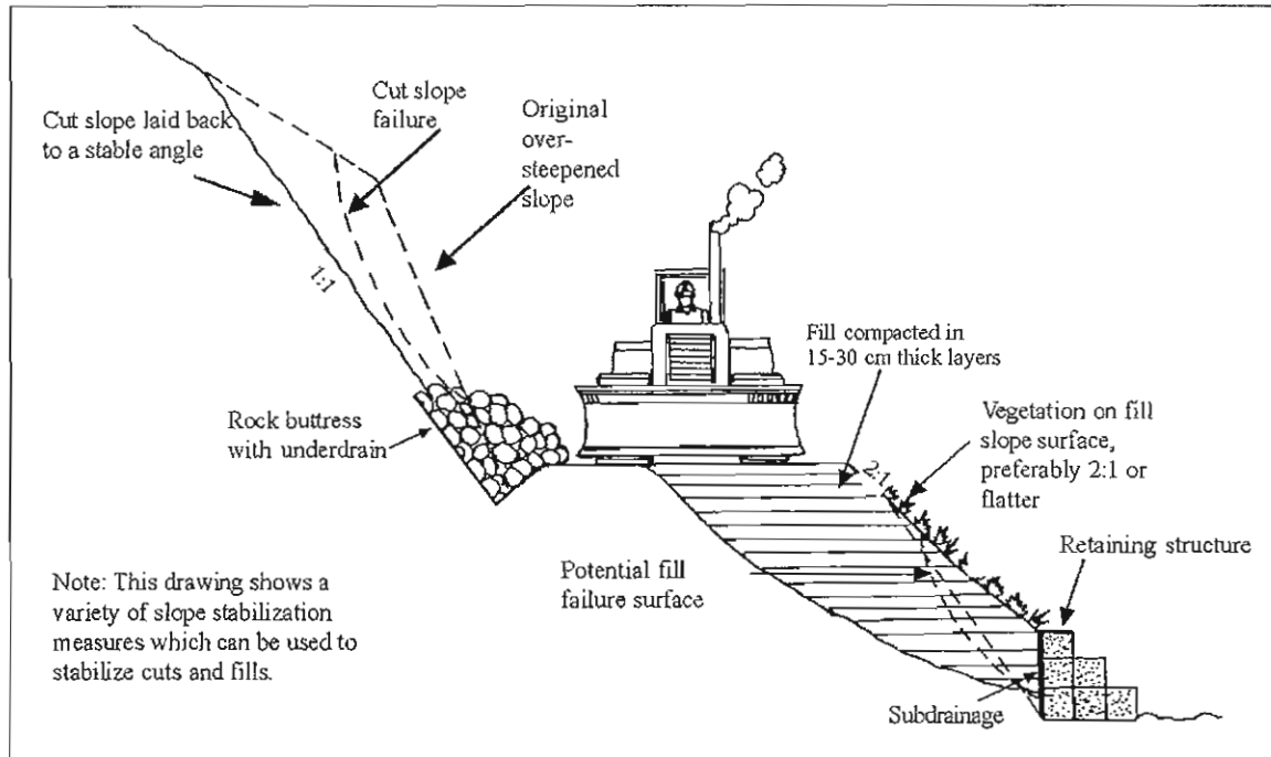
Figure 2. Slope Stabilization Detail with Rock Butress
