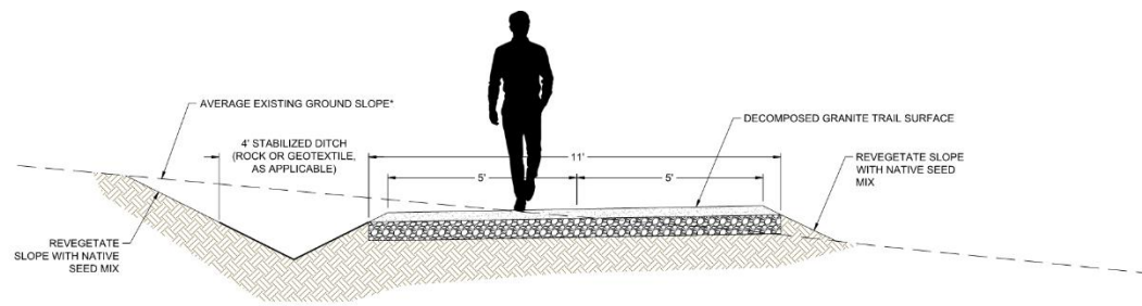
TYPICAL TRAIL SECTION N.T.S.
